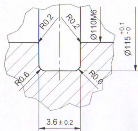
A (5:1)
