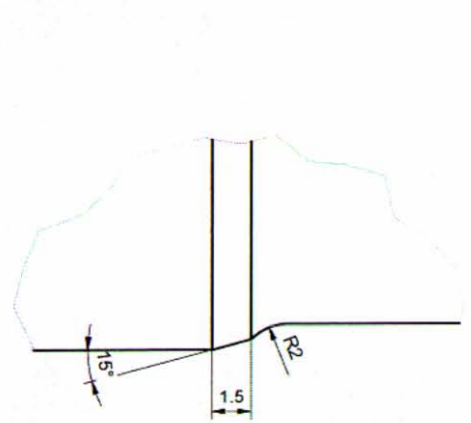
D (5:1)
